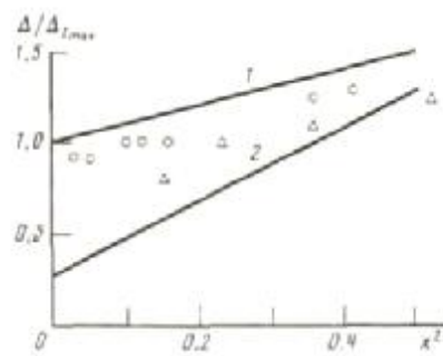
FIG. 3. Dependences of the half-widths of the lines of the observed signal on the intensity of the exciting field: 1) I_{\perp} ; 2) I_z (theory); O, Δ) experimental results for I_{\perp} and I_z , respectively. The ordinate gives the half-width in units of 1/T_2 .
