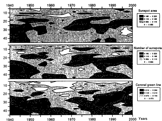
Figure 6. SVAN diagrams (from top to bottom) for the asymmetry in different activity indices for the sunspot formation zone of 0^{\circ} - 30^{\circ} .
