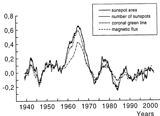
Figure 2. Long-term asymmetry variations in four activity indices in the sunspot formation zone 0^\circ - 30^\circ .
