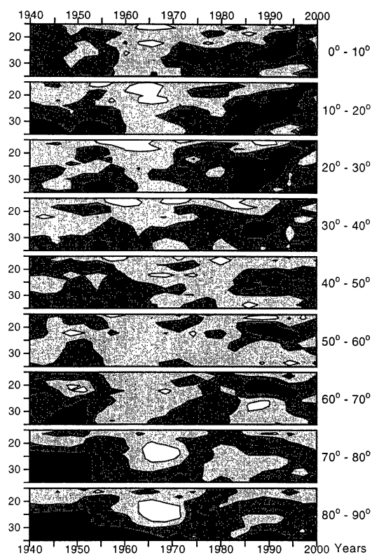
Figure 4. Spectral-Variation Analysis (SVAN) of the N-S asymmetry in the coronal green line brightness.
