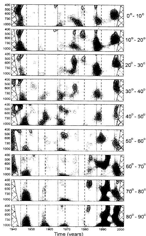
Figure 5. Wavelet analysis of the N-S asymmetry in the coronal green line brightness.
