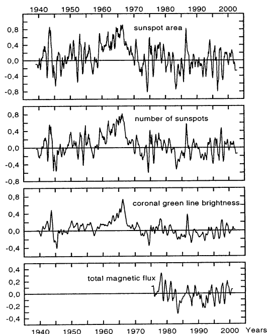
Figure 1. Asymmetry variation in four solar activity indices in the sunspot formation zone 0^\circ - 30^\circ .
