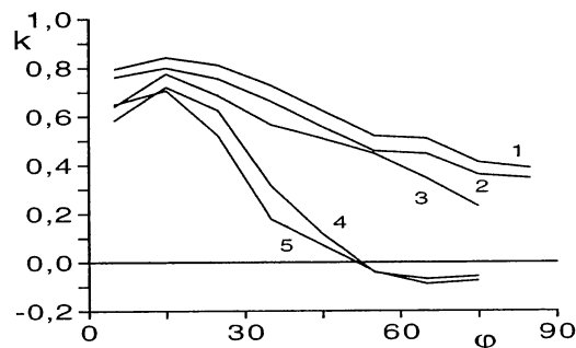
Figure 3. The mutual correlation of the semi-annual mean asymmetry values of different solar activity indices as a function of latitude.
