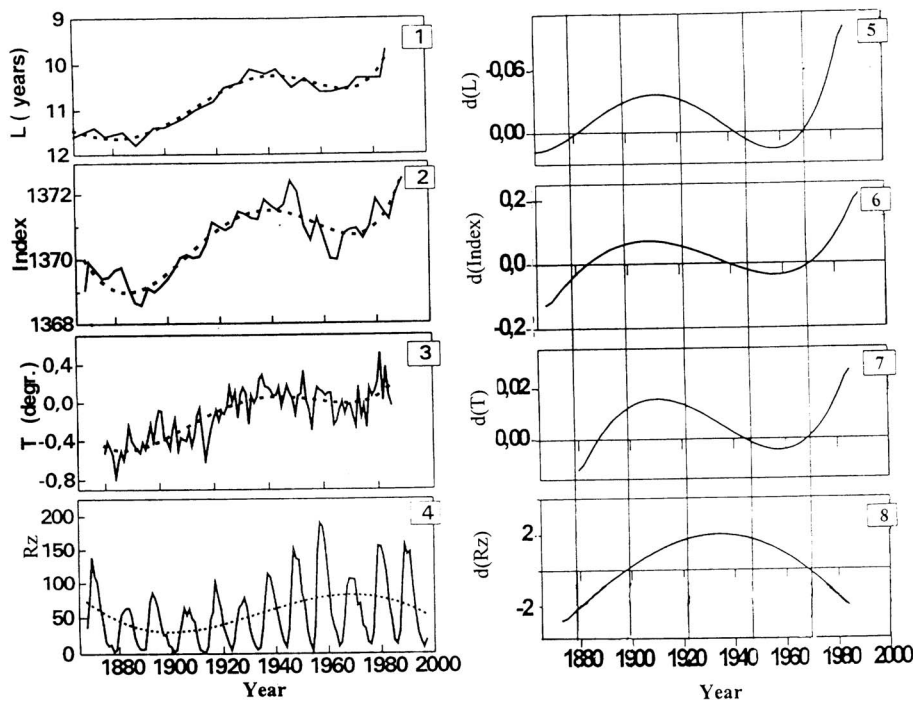
Fig. 11. Left column: variations of the sunspot cycle length — panel 1, the Hoyt and Schatten (1993) composite solar irradiance index (based upon five solar indices, namely cycle length, cycle decay rate, mean level of solar activity, solar rotation and the fraction of penumbral sunspots) — panel 2, northern hemisphere land-air surface temperature anomalies from 1868 to 1990 — panel 3, and the sunspot number — panel 4. Sixth order polynomial fits are shown by dashed lines. Right column: the derivatives of sun-spot cycle length — panel 5, of the Hoyt and Schatten (1993) composite index — panel 6, of the northern hemisphere land-air surface temperature anomalies — panel 7, and of the solar sunspot numbers — panel 8. The times of low solar-geomagnetic correlation are shown by vertical straight lines.
