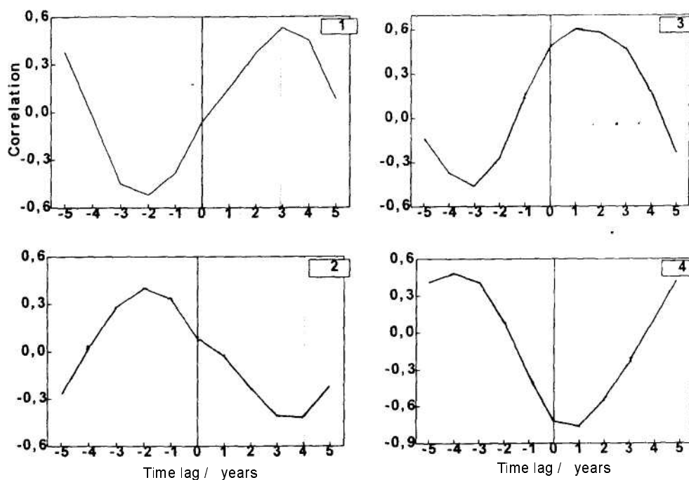
Fig. 8. Examples of the crosscorrelation functions for two 23-year periods with the low (1966-1988) (panels 1 and 2) and high (1947-1969) solar-geomagnetic correlation (panels 3 and 4). Panels 1 and 3 correspond to crosscorrelation between R_z and T(aa \geq 30) , and panels 2 and 4 between R_z and T(aa \leq 4) .
