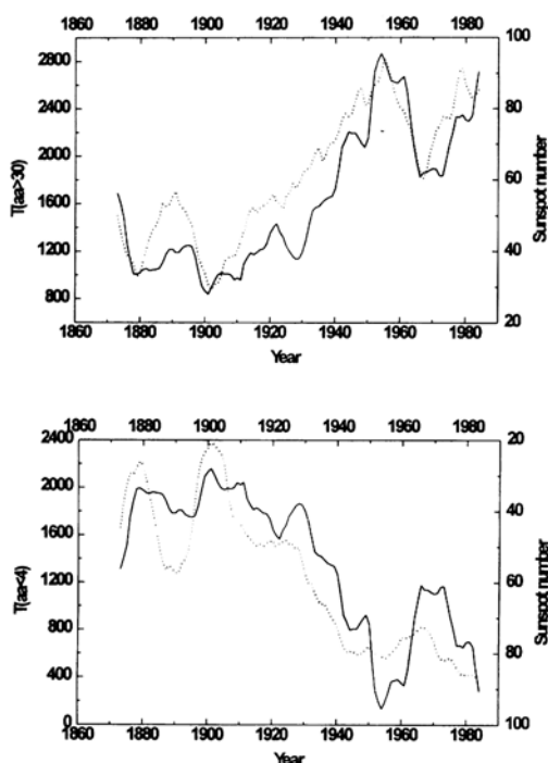
Fig. 4. Top panel — low frequency components of R_z (solid line) and T(aa \geq 30) (dots) filtered by the 11-year running mean. Bottom panel — the same components of R_z (solid line) and T(aa \leq 4) (dots).
