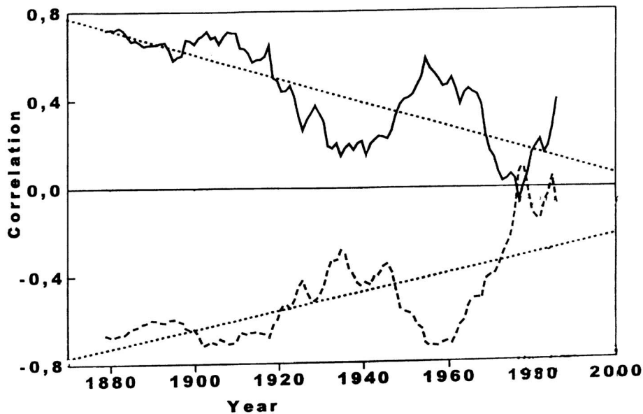
Fig. 3. The 23-year running-window correlation between R_z and T(aa \leq 4)/T(aa \geq 30) : R_z and T(aa \leq 4) dashed line, and R_z and T(aa \geq 30) solid line. Linear regression fits are shown by dots.
