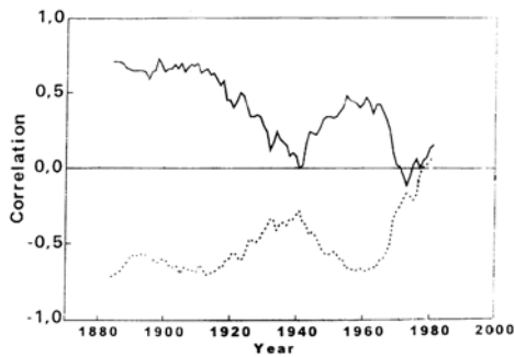
Fig. 6. The 23-year running-window correlation between high frequency fluctuations of R_z and T(aa \leq 4) dashed line, and between the same fluctuations of R_z and T(aa \geq 30) solid line.
