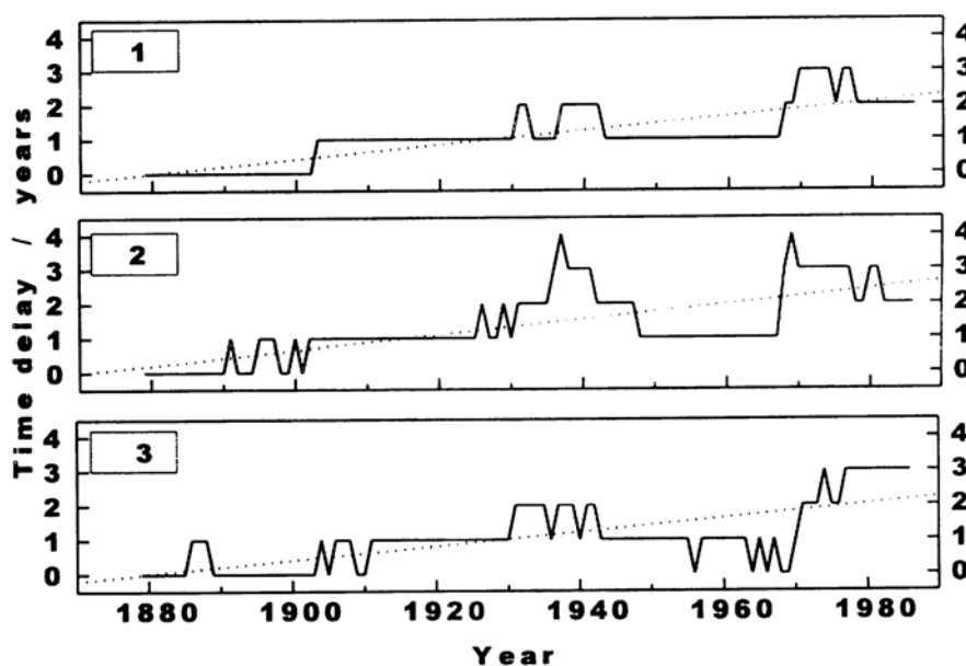
Fig. 9. Long-term variations of time delay of the following geomagnetic indices relative to sunspot numbers: panel 1 — aa , panel 2 — T(aa \geq 30) , panel 3 — T(aa \leq 4) . Linear regression fits are shown by dots.
