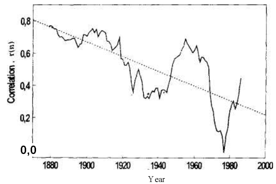
Fig. 1. The 23-year running-window correlation between R_z and aa-indices. Linear regression fits are shown by dots.
