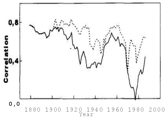
Fig. 10. The 23-year running-window correlation between R_z and aa corrected for shifts of maxima of the crosscorrelation functions (points) and without correction (solid line).
