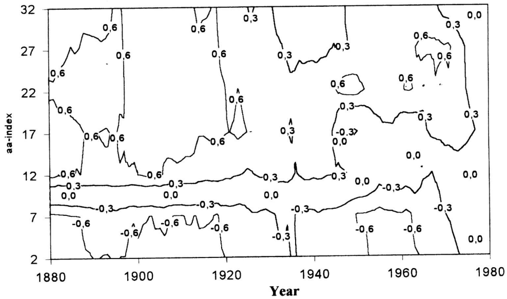
Fig. 2. The field of isolines of the 23-year running-window correlation between R_z and T(aa,2) over the entire range of aa values.
