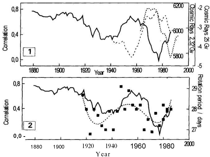
Fig. 12. Panel 1 — the long-term variations of the solar-geomagnetic correlation (solid lines) and parameters of galactic cosmic rays: the variations of Kiel (Germany) neutron monitor pressure-corrected counting rate for 2.32 GV cutoff rigidity (points), and density of galactic cosmic rays for 25 GV rigidity relative to the level in 1965, calculated from the worldwide cosmic ray network stations (dashed line), smoothed by 11-year running mean. Panel 2 - the variations of rotation period of the Sun's large-scale magnetic fields, obtained by Obridko and Shelting (1998) (squares), together with their sixth order polynomial fit (dots) and the long-term variations of solar-geomagnetic correlation (solid line).
