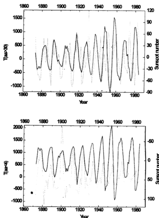
Fig. 5. Top panel — high frequency fluctuations of R_z (solid line) and T(aa \geq 30) (dots) with periods no greater than 11 years. Bottom panel — the same fluctuations of R_z (solid line) and T(aa \leq 4) (dots).
